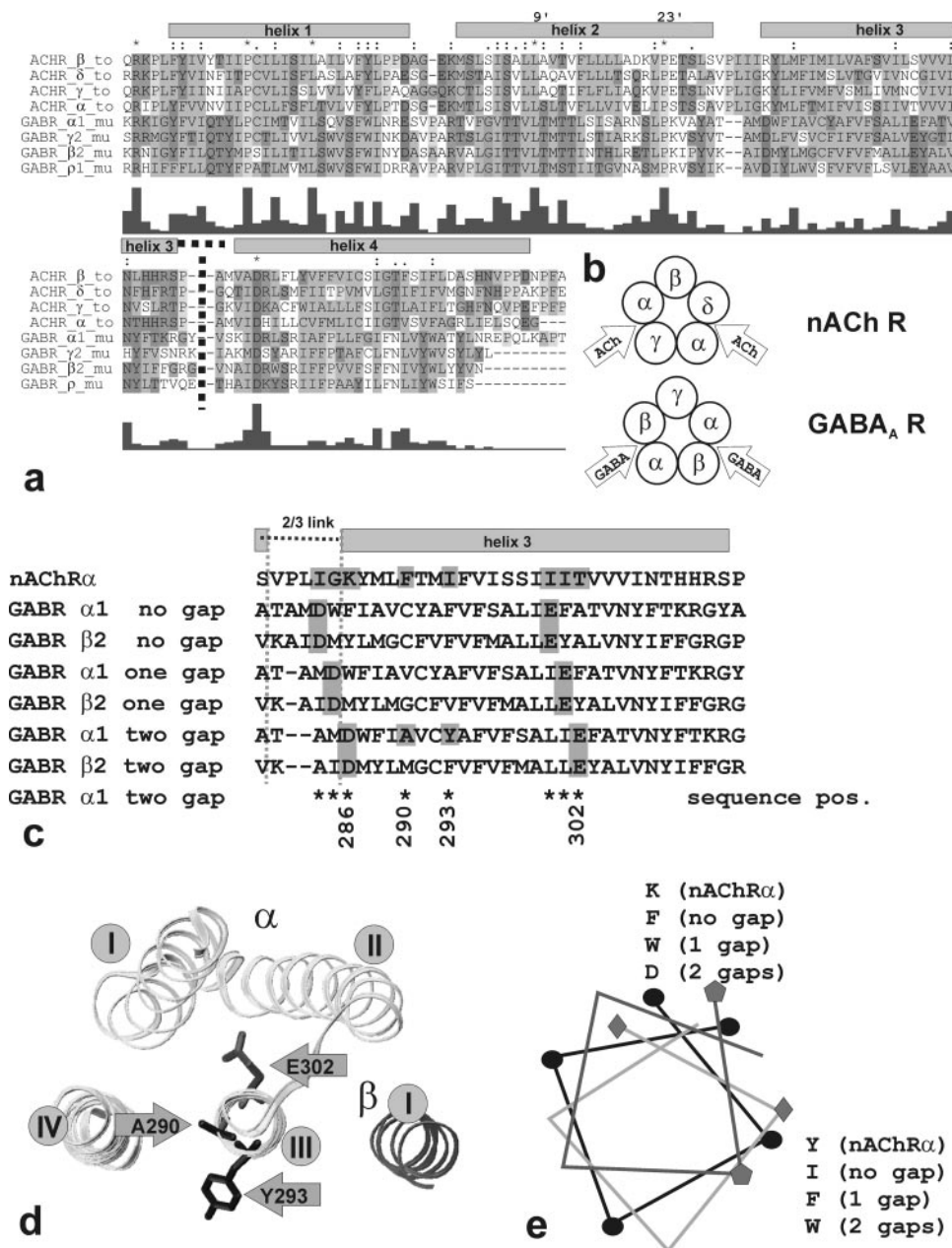
Fig. 1. Alignment of nACh and GABA A receptor helical domains. a , a subset of a superfamily alignment of the four segments that make up the helical (transmembrane) domain of the subunit chains is shown. The position of the missing "cytoplasmic loop" between helices 3 and 4 is indicated by a double-gap and a bold dotted line across all columns. Note that for helices 3 and 4, other alignment variants can be found, depending on the alignment parameters and on the number and choice of sequences that are included in a multisequence alignment. Standard Clustal (Thompson et al., 1997) symbols (*,.) are used to indicate degree of sequence conservation, also indicated by the bar graph beneath the alignment. b , subunit correspondence between nACh receptors and GABA A receptors is indicated by the schematic pentamers; arrows indicate agonist binding site locations. c , three different alignments for helix 3 of GABA A receptor \alpha_1 and \beta_2 subunits with the corresponding nACh receptor \alpha subunit segment from 10ED are shown. They result from placing zero, one, or two gaps in the alignment of the 2/3 linker between cation and anion channels. GABA A receptor residues \alpha_1 Asp286 and \alpha_1 Glu302, corresponding to a conserved Asp and Glu in anion channels, are highlighted to emphasize how they align with residues in the nAChR in the three alignment variants. The highly solvent accessible nACh receptor residues \alpha Phe280 and \alpha Ile282, as well as GABA A receptor residues \alpha_1 Ala290 and \alpha_1 Tyr293, which can be cys-modified in appropriate mutants in the resting state, are also highlighted. d , model corresponding to the two-gap alignment of helix 3 of a GABA A receptor \alpha subunit. Helix 3 is viewed from the N terminus and perpendicular to the paper plane, and all neighboring protein segments are also shown. Approximate side-chain orientations for the two cys-modifiable positions \alpha_1 Ala290C and \alpha_1 Tyr293C (wild-type side chains shown) are depicted, as well as the position for \alpha_1 Glu302 that is modifiable only under gating conditions. e , the helical wheel of the utmost N terminus of helix 3 is shown as schematic C- \alpha trace; the black trace indicates the nACh receptor. The residue correspondence according to the three alignment variants shown in c is indicated for the first two helix positions. Natural variation in C- \alpha position of distant homologs is indicated by two additional (gray) alternative helical wheels; the first two C- \alpha atoms are indicated by different symbols. The indicated deviations correspond to C- \alpha position changes in the order of 2 Å. Deviations of up to 5 Å are possible in structurally corresponding residue positions in homologs of low sequence identity.
